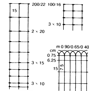
② Twisted link and decorative lattice
